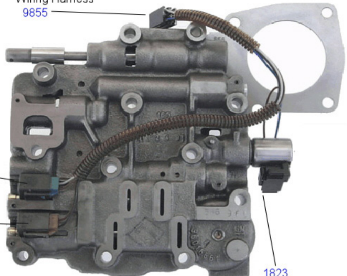
1823 PWM Band Control Solenoid
